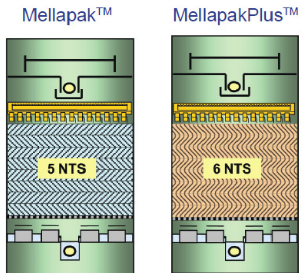
Typical Application of MellapakPlus™ with 20% more Efficiency
